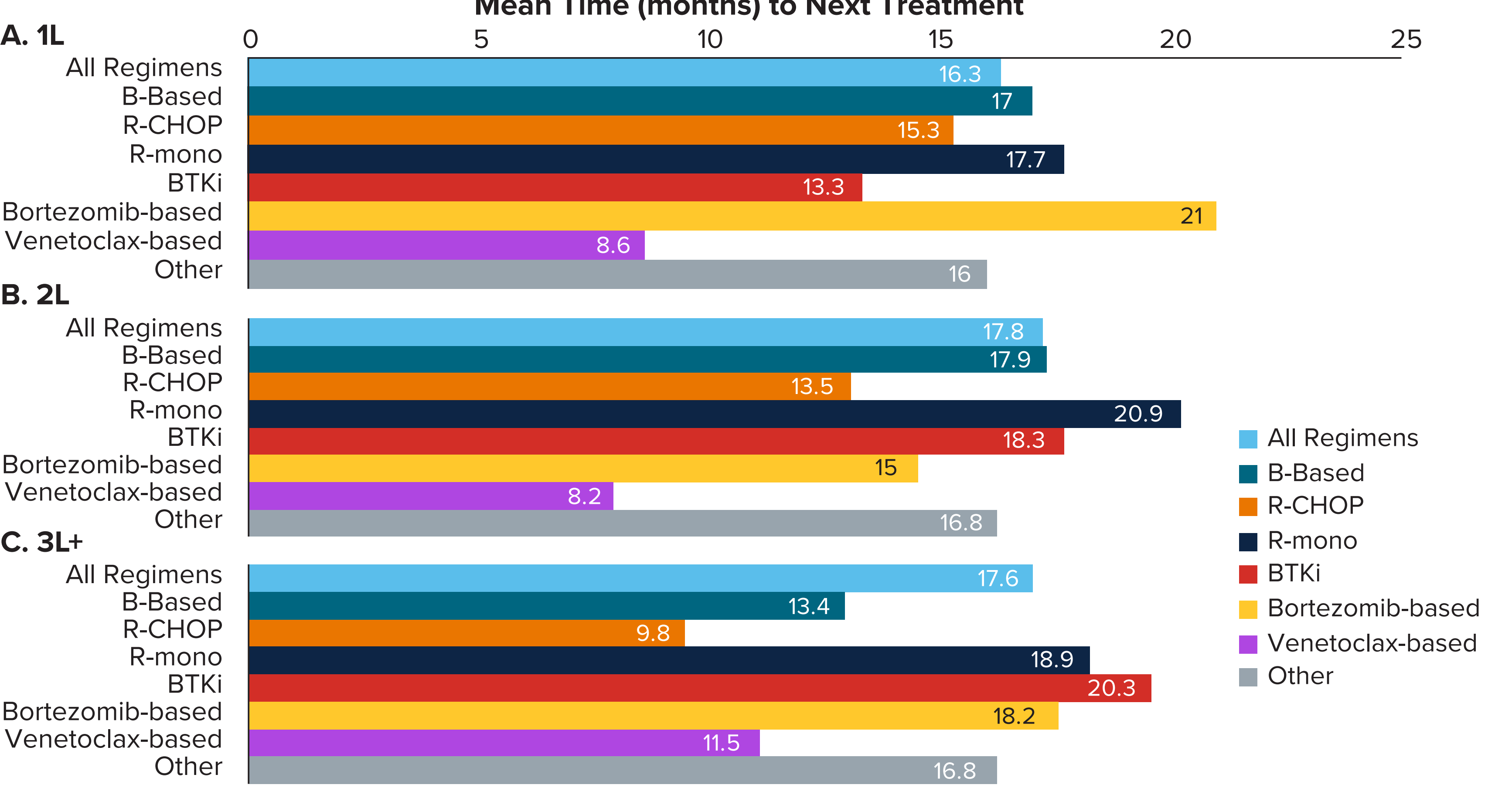
Figure 2. Mean TTNT
